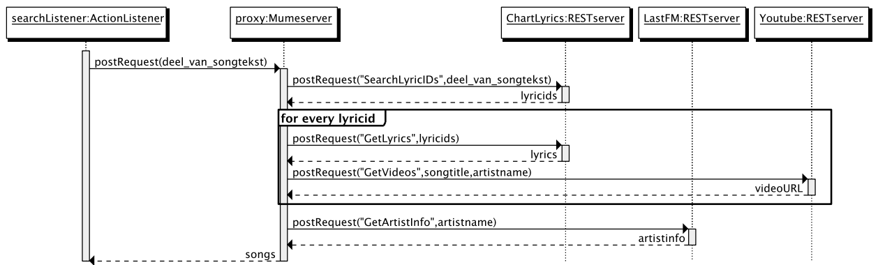
Figuur 6: Server Communication
