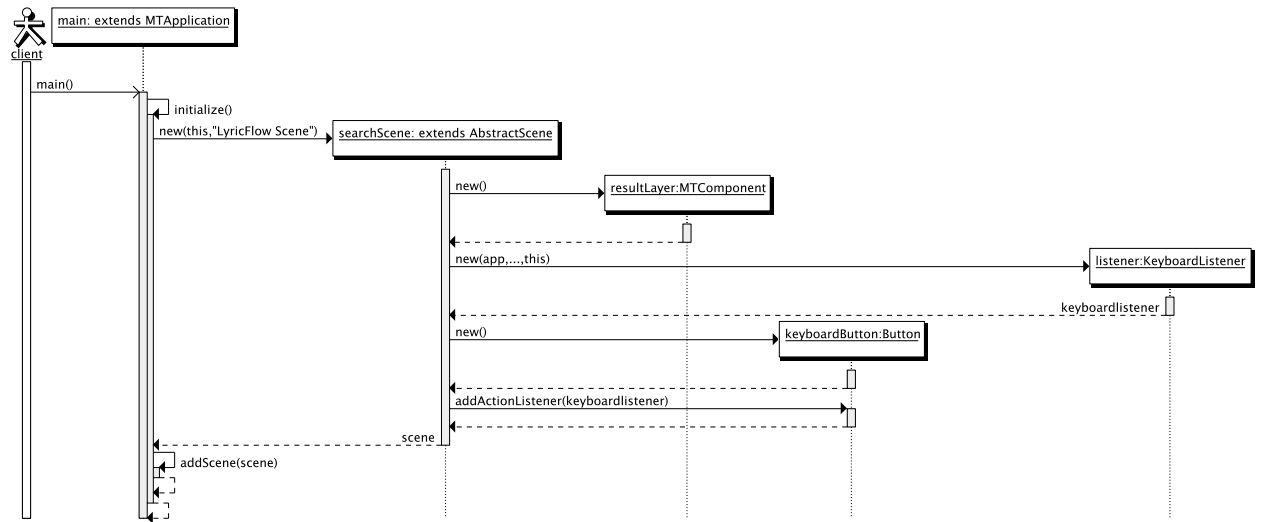
Figuur 3: Keyboard Creation
